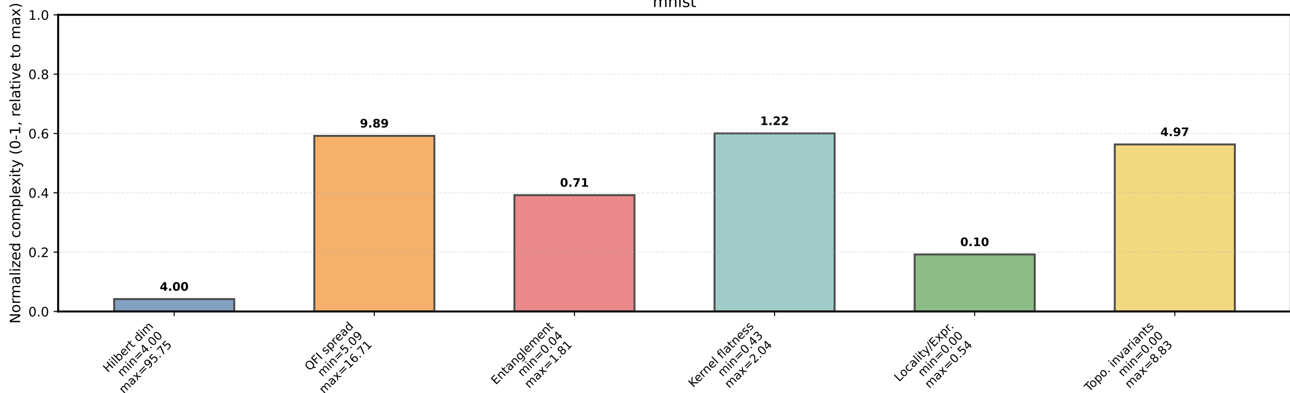
Complexity metrics for dense amplitude encoding mnist
